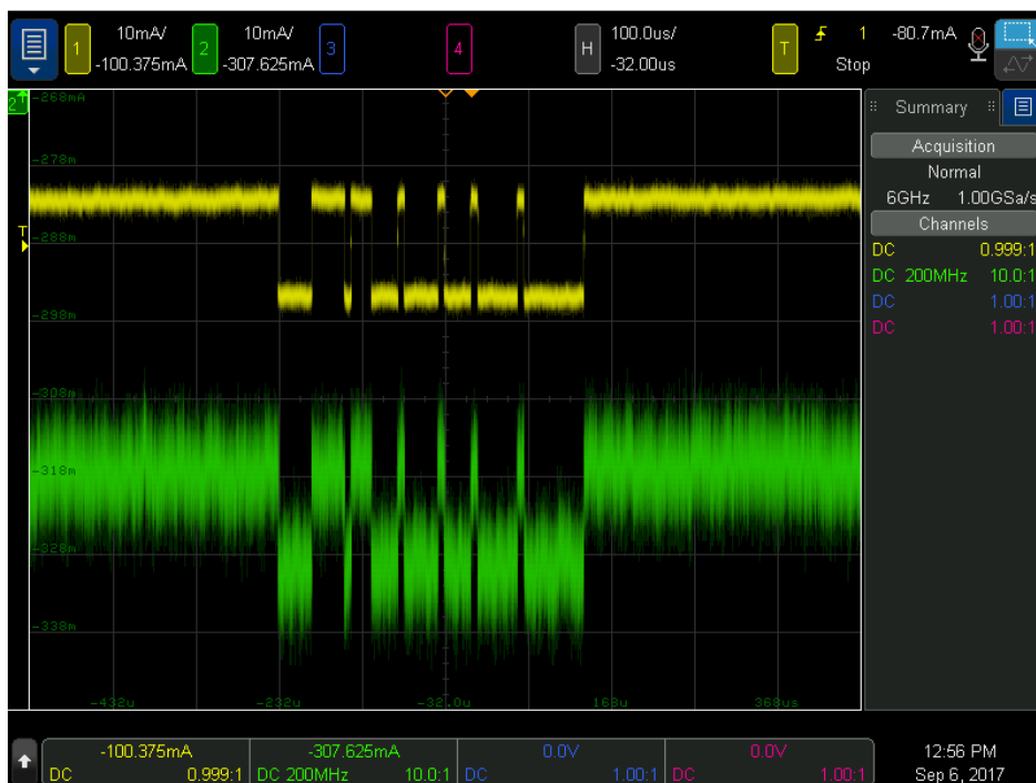
Improved noise floor of the N7026A (yellow trace) over the N2893A (green trace)
