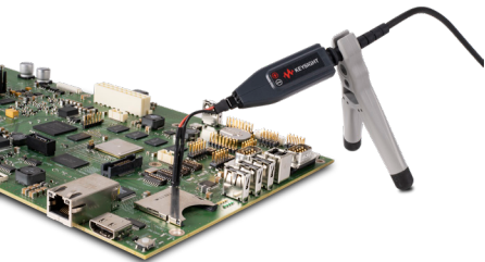
DP001xA Series probe using socketed Y-lead
