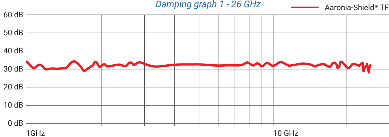
Damping graph 1 - 26 GHz
