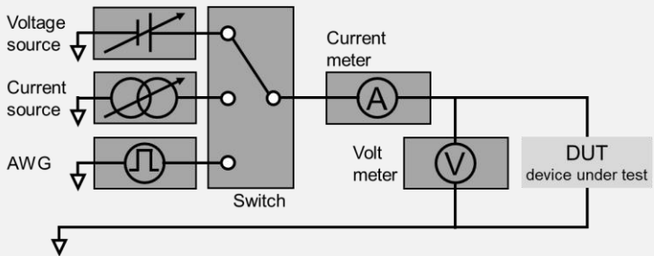
Rack & stack solution: Multiple instruments connected with no easy means to coordinate them.
