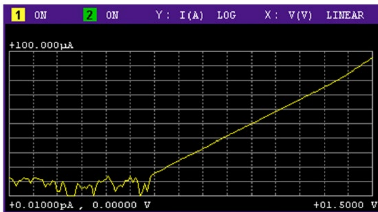
Figure 3. You can make and display accurate low-current measurements directly on the B2900C/CL front panel.
