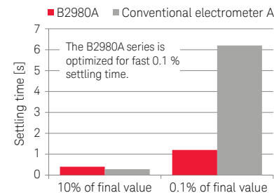
20 pA range settling time 2 V step, 100 GΩ, 1 PLC
