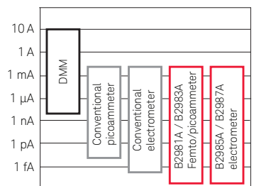
Typical current measurement ranges
