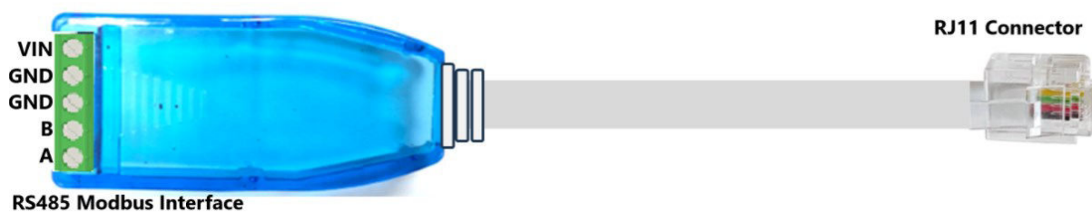
Figure 5 - RS485-RJ11 Cable(30cm)
