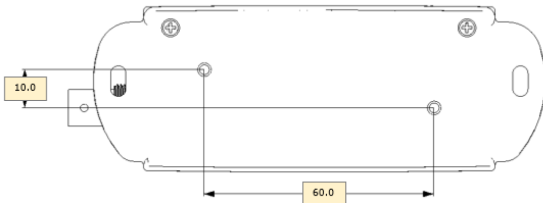
Figure 8 - Modbus ORP Sensor Adapter Dimension – Bottom View
