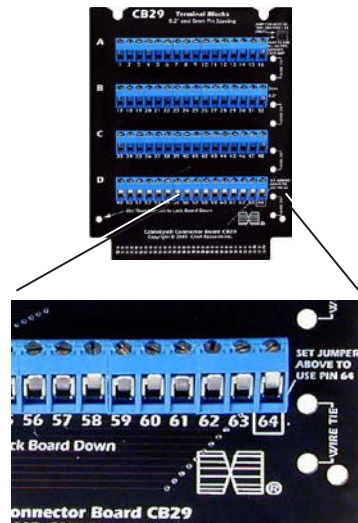
Close-Up of Terminal Block
