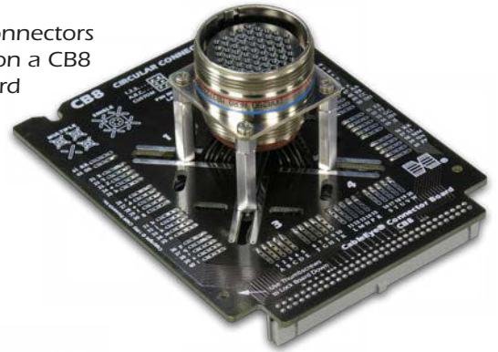
Back Panel Testing with Flat and AMPMODU Mating Adapters
