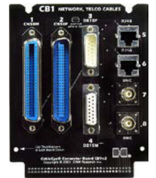
CB1 CN50, DB15 RJ45, BNC (Item 731)
