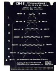
CB43 Micro D Connectors, 9- through 37-Pin (Item 773)
