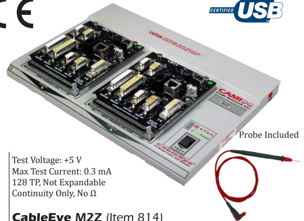
CableEye M2Z (Item 814) shown with CB15C Boards (Item 745C) Installed
