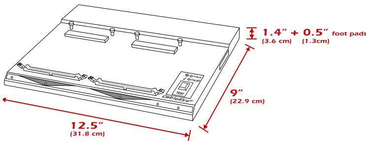
Dimensions for low voltage testers.
