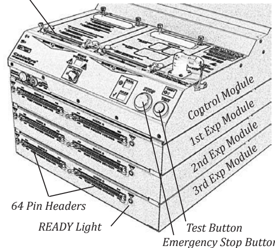
HVX System with Three Expansion Modules
