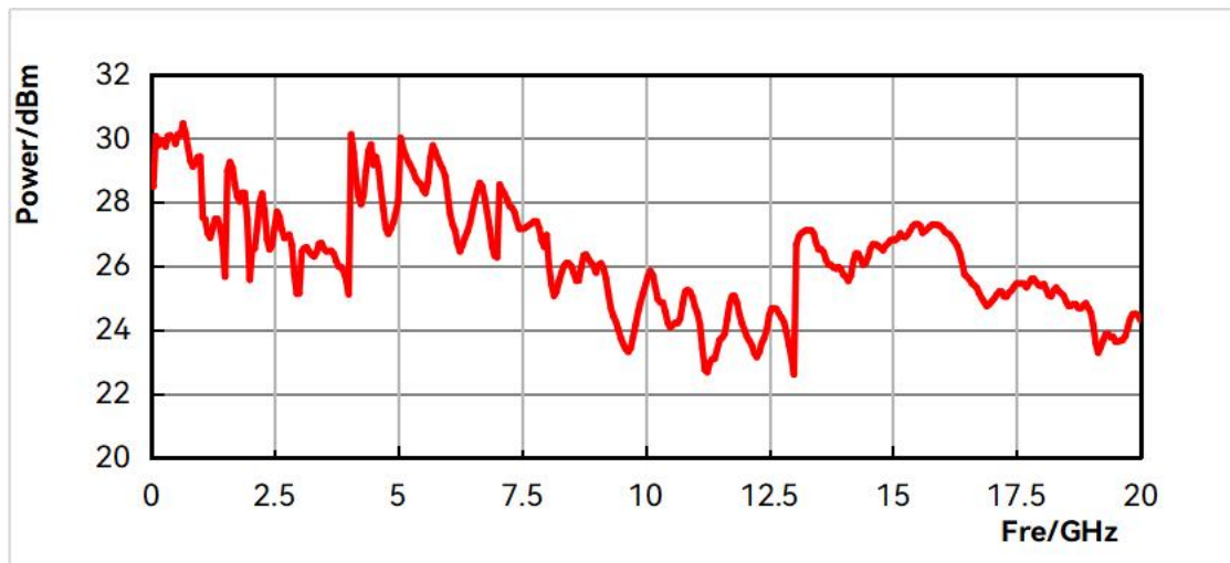
1466D-V: measured max. output power (option H05-20)
