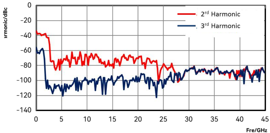
1466G-V: measured harmonic
