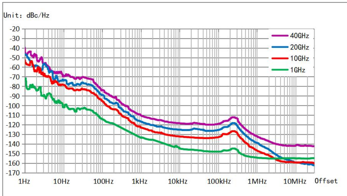
Option H04-2: measured SSB phase noise
