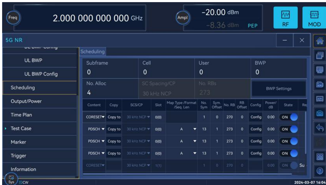
Downlink scheduling Settings
