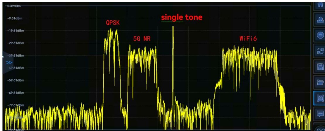
Different modulation types of multi-carrier test map
