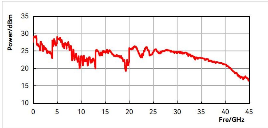
1466G-V: measured max. output power (option H05-45)
