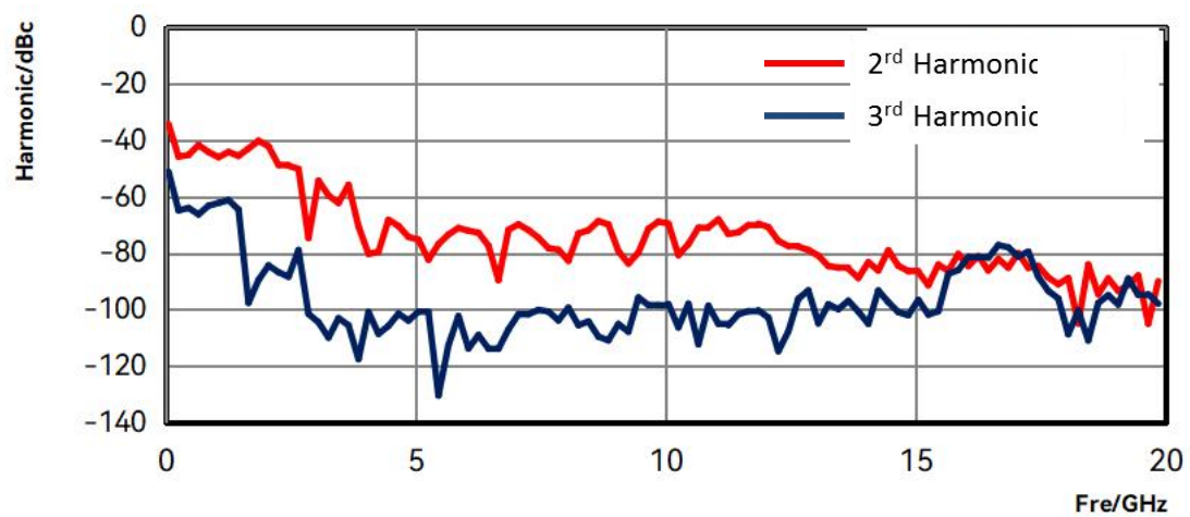
1466D-V: measured harmonic
