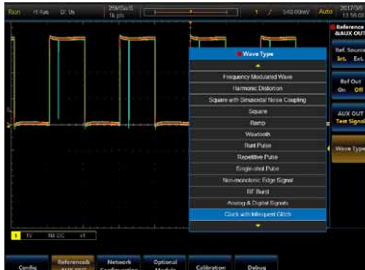
Test signal: runt pulse signal
