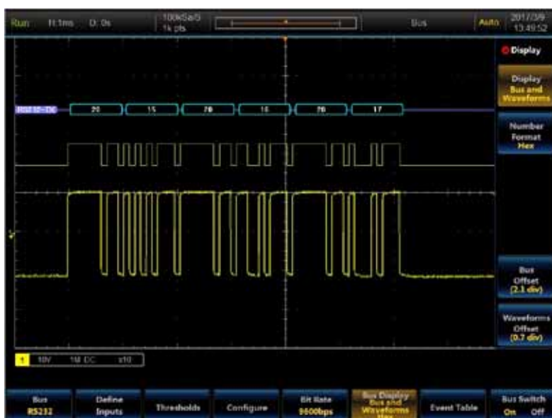
Computer bus: RS232, USB
