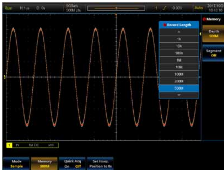
500Mpts/CH deep storage, maintains high sample rate in a long sample period.
