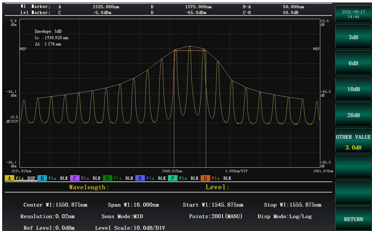
Center wavelength and bandwidth test based on envelope analysis
