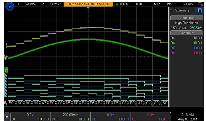
Figure 24. Optional digital channels allow a timing view of up to 16 channels. Tightly integrated, they work with the analog triggers and serial triggers/decoding.
