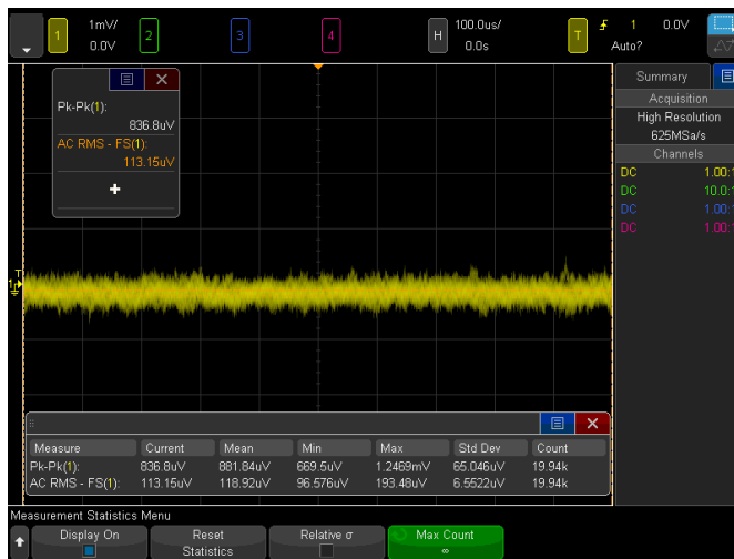
Figure 40. Getting 113 \mu\text{Vrms} noise floor at 1 mV/div with the high-resolution mode.
