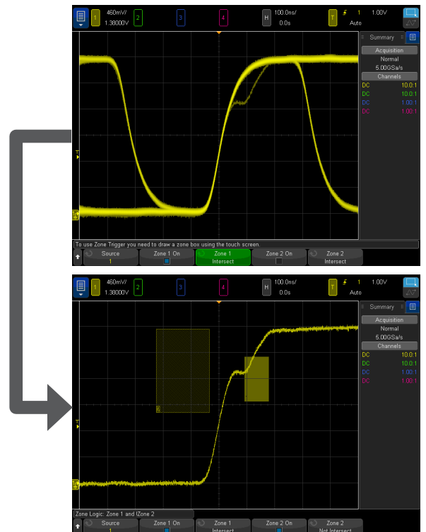
Figure 15. When you see anomalies, all you have to do is draw a zone box to trigger on them.
