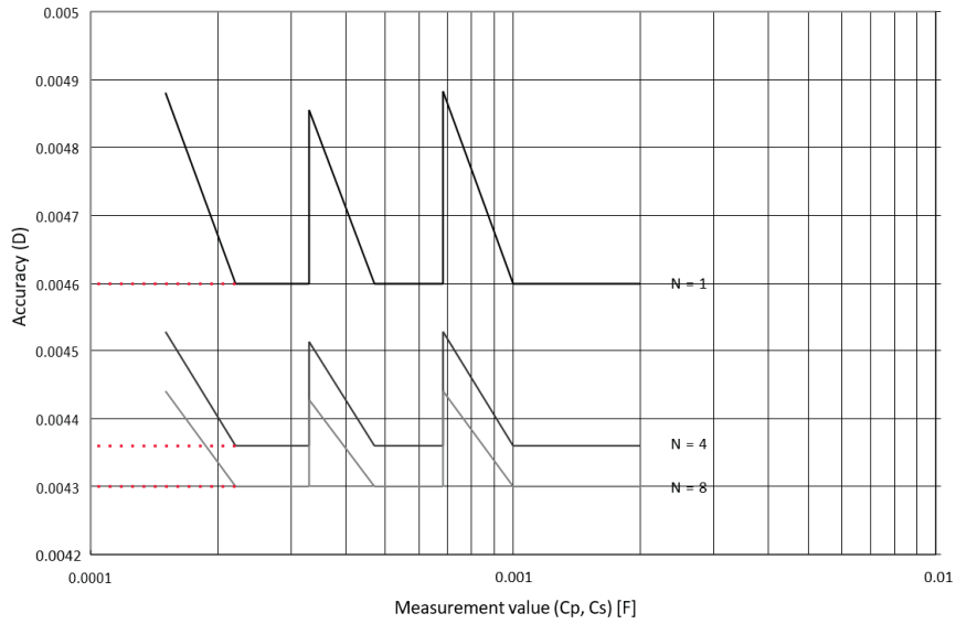
Figure 3. Accuracy of D when measurement frequency is 120 Hz (measurement range: 220 \mu F to 1 mF / measurement signal level: 1 V)
