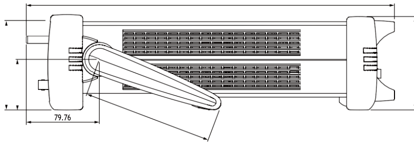
Figure 19. Dimensions (side view, with handle and bumper, in millimeters, nominal)
