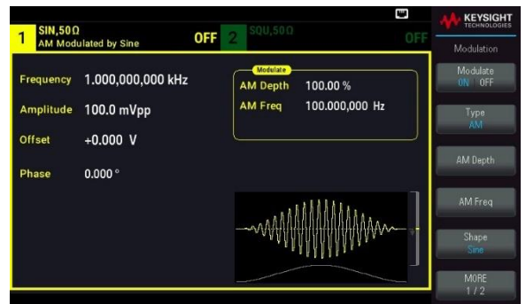
Figure 4. AM modulated with a standard sine wave
