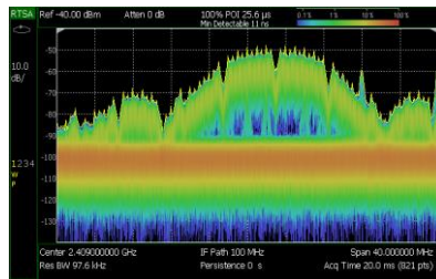
Identify multiple types of signals within the same frequency band
