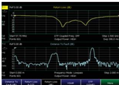
View return loss and DTF simultaneously
