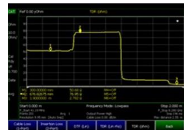
Gain insight into faults with TDR measurement
