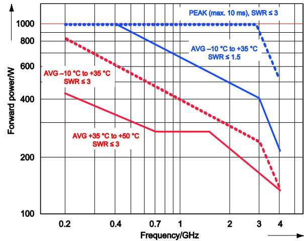
Power-handling capacity
