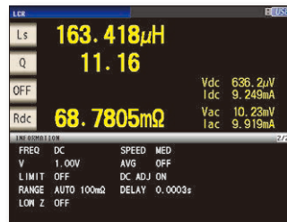
L/Q/ Rdc continuous measurement screen (1 kHz, 1 mA constant current measurement) and Rdc (DC measurement) display screen
