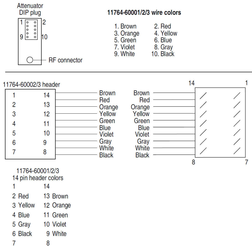
Figure 4. Attenuator switching pinout
