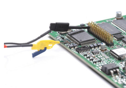
IC clips included in N2877A and N2878A accessory kits for N2870A Series passive probes
