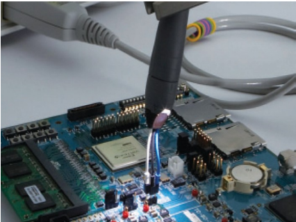
InfiniiMode probe with either socketed tip or solder-in tip allows convenient measurements of differential, SE and CM signals with a single probe. Probe head light is built-in
