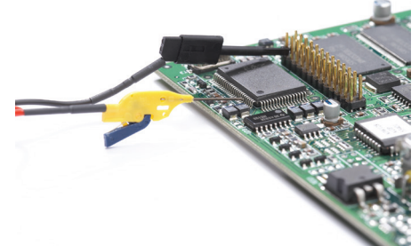
IC clips included in N2877A and N2878A accessory kits for N2870A Series passive probes
