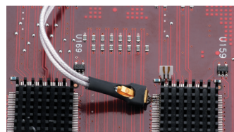
N5439A InfiniiMax III ZIF probe head soldered in to an IC
