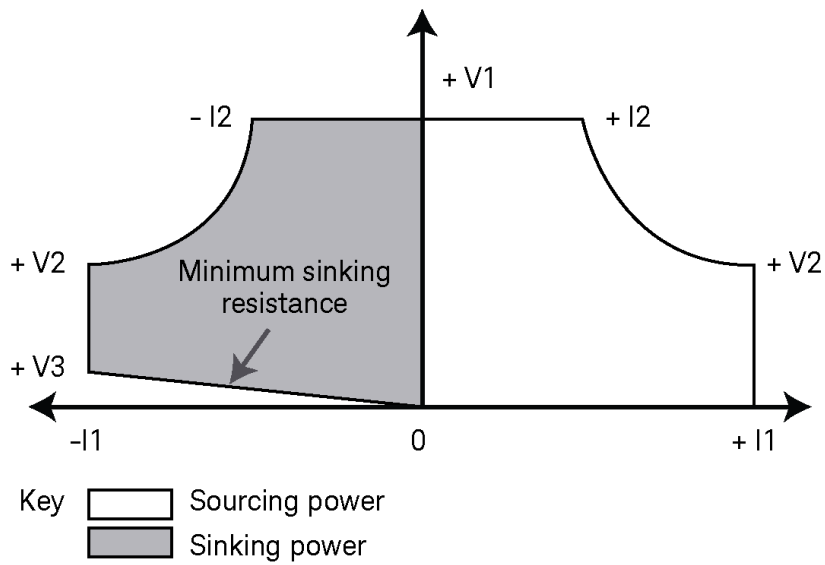
Figure 7. RP5900 output characteristic
