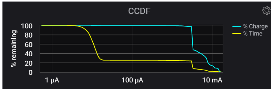
Figure 11. Complementary Cumulative Distribution Function (CCDF).
