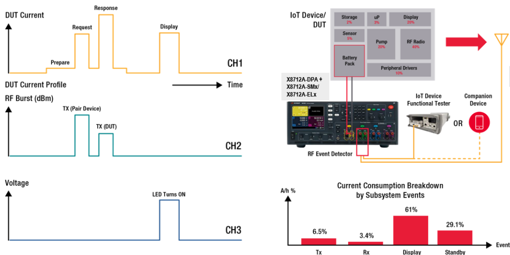
Figure 2. The X8712A event-based power analysis concept
