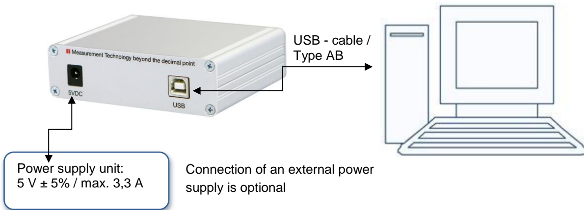
Figure 12: Connection of USB hub to the PC
