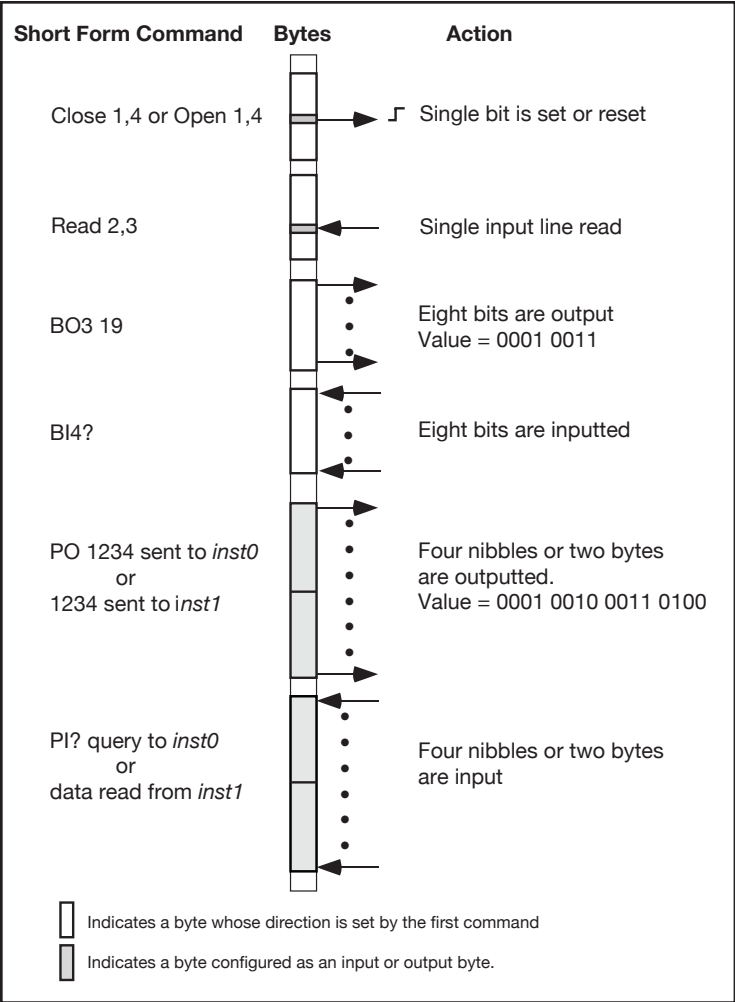
Figure 2 8063 Digital Interface Data Transfer Methods (Figure shows 8 bytes for illustrative purposes. Actual 8063 has 6 bytes)
