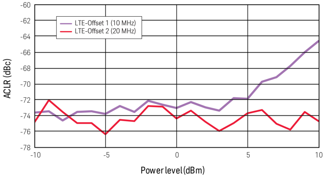
Measured 10 MHz LTE E-TM 1.1 QPSK ACLR (with Option UNV + 1EA)
