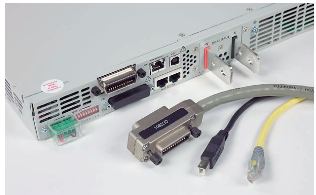
Figure 2. Built-in Ethernet, USB 2.0, and GPIB interfaces enable easy system connections.
