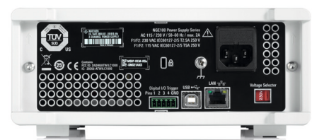
Rear view of the R&S®NGE100B series
