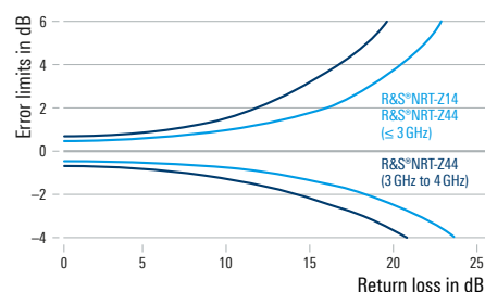
Measurement error limits (two standard deviations) for reflection measurements with the R&S®NRT-Z14/-Z44 directional power sensors
