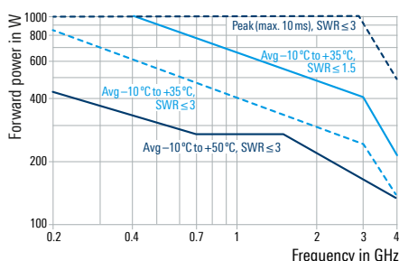
Maximum forward power of the R&S®NRT-Z44 directional power sensors (for both directions)
