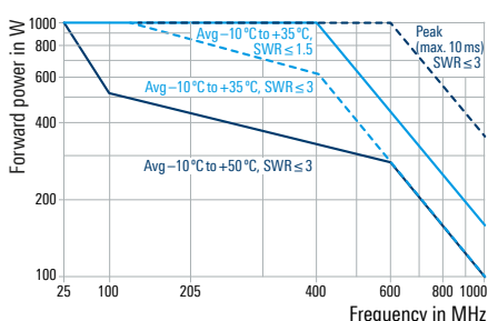
Maximum forward power of the R&S®NRT-Z14 directional power sensor (for both directions)
