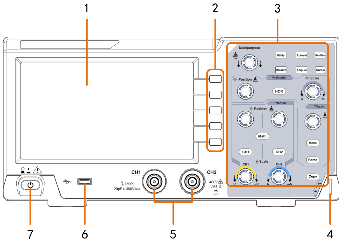
Figure 1-1 Front panel
