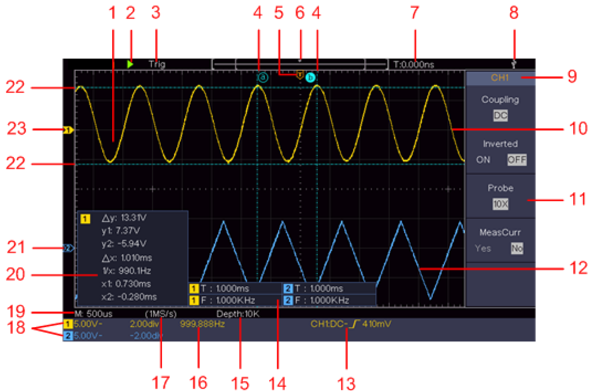
Figure 1-4 Illustrative Drawing of Display Interfaces
