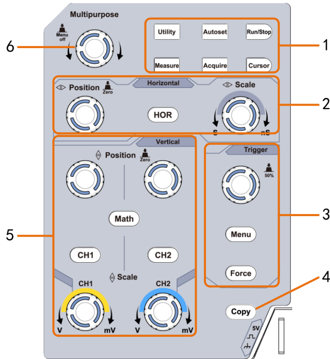
Figure 1-3 Control Area Overview
