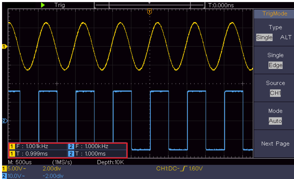
Figure 0-6 Automatic measurement
