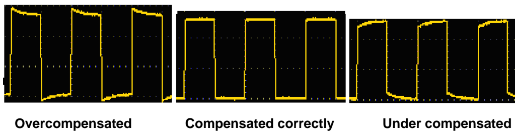
Figure 1-6 Displayed Waveforms of the Probe Compensation
