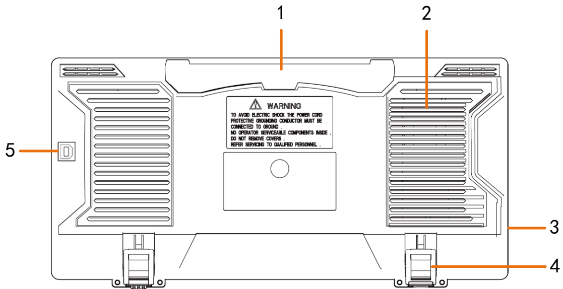
Figure 1-2 Rear Panel
