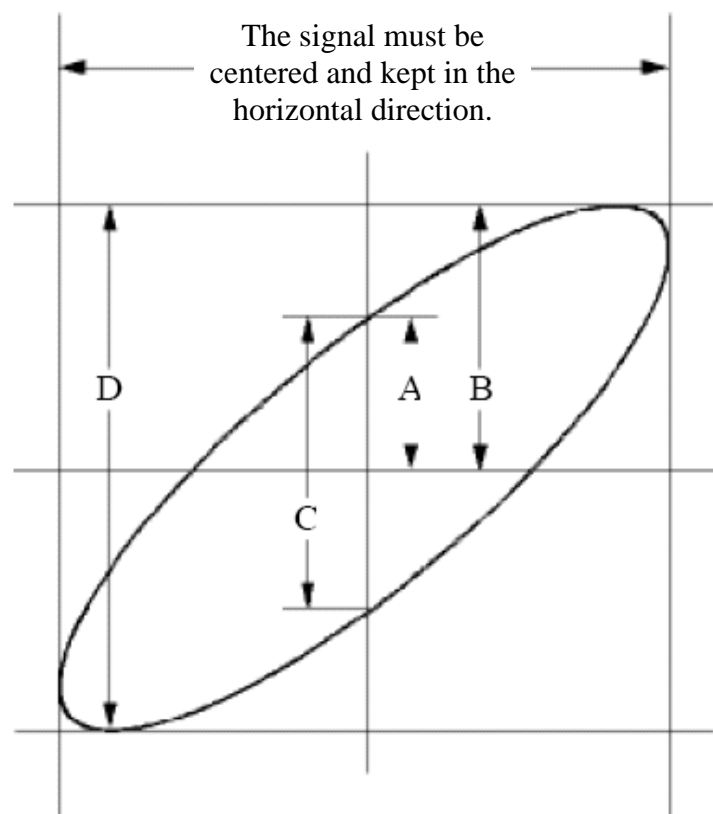
Figure 0-6 Lissajous Graph
