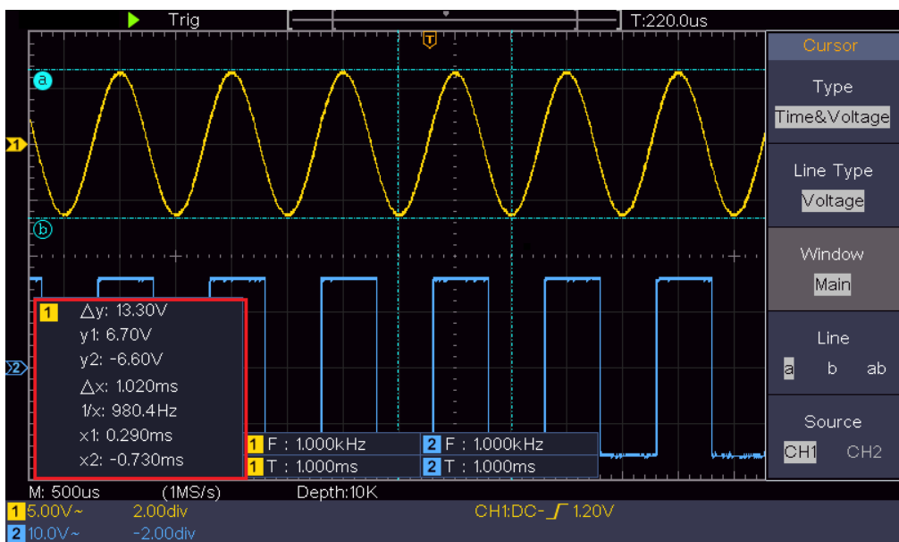
Figure 0-9 Time&Voltage Cursor Measurement
