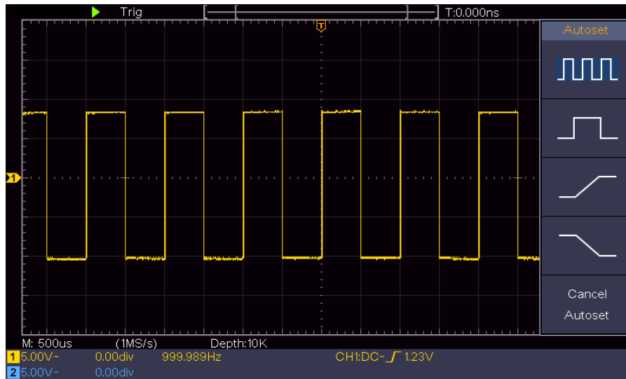
Figure 1-5 Auto set
