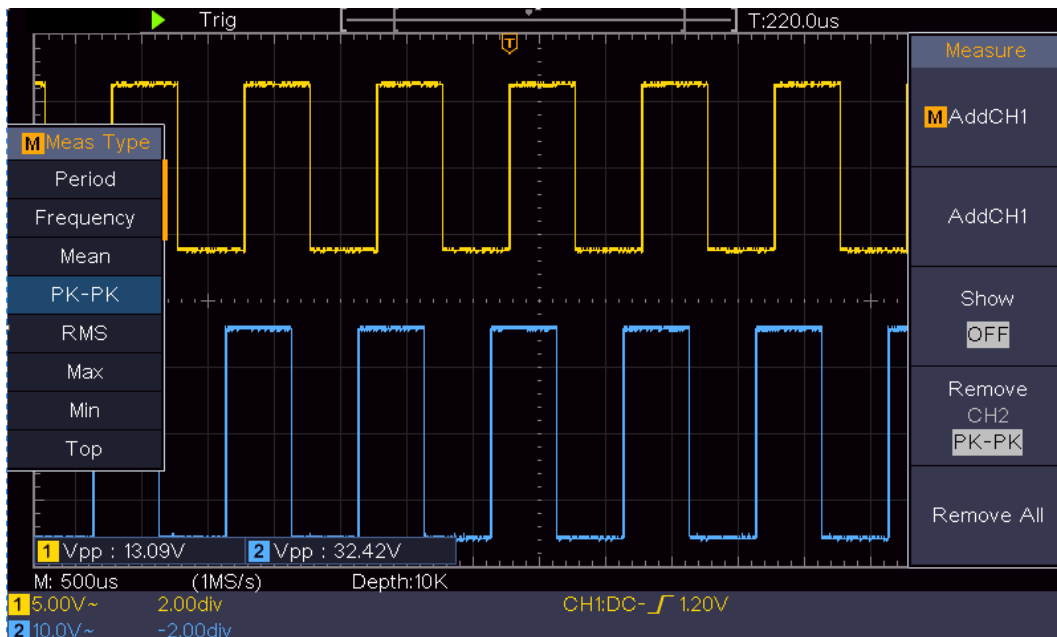
Figure 0-2 Waveform of Gain Measurement
