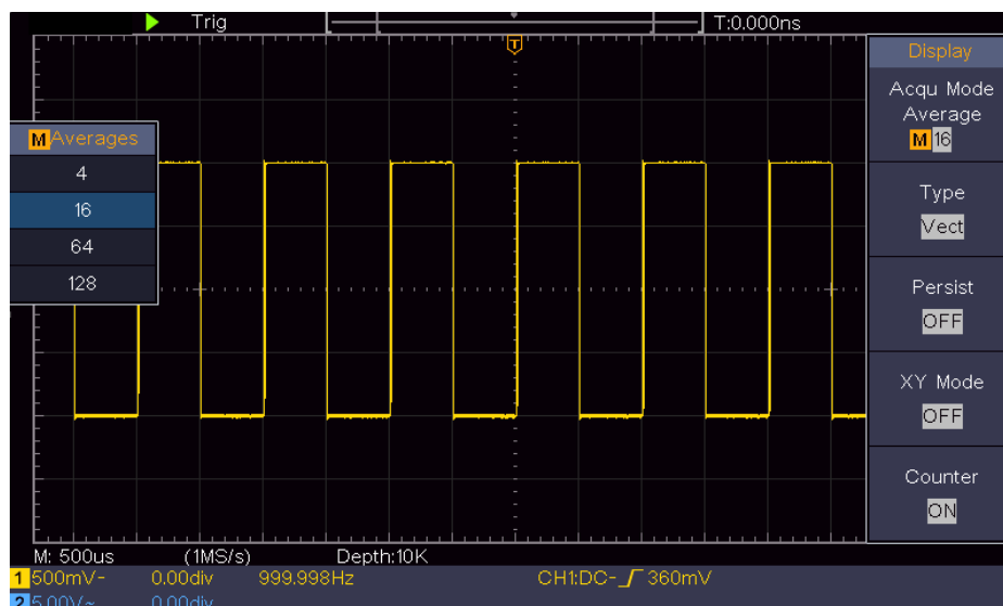
Figure 0-5 Reduce Noise level by using Average function
