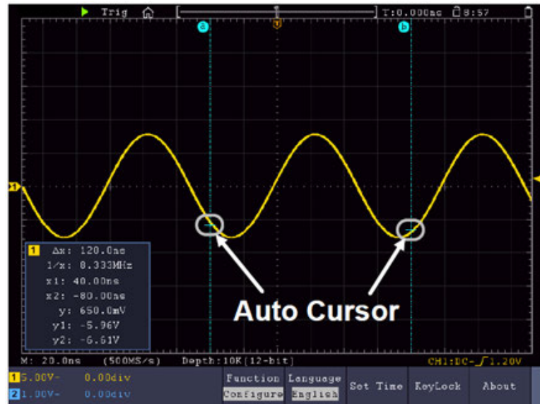
Figure 4-21 Auto Cursor
