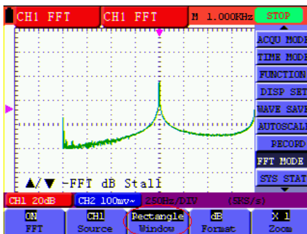
Figure 55: Rectangle window
