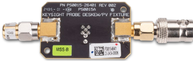
Figure 8. Deskew and performance verification fixture (PS0015A) with SMA and BNC adapters
