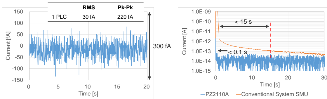
Measurement noise, 10 nA range, no load, 0 V, triax cable (3 m)
