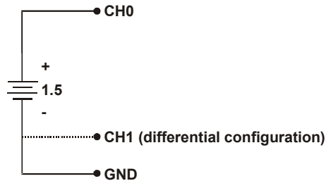
Figure 6. Single-ended measurement connection
