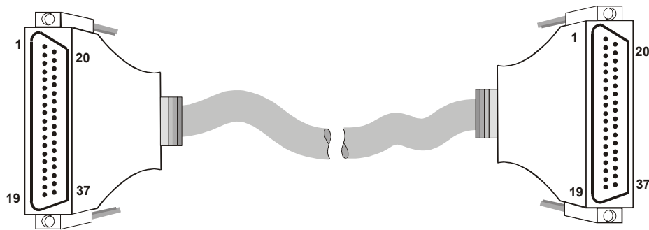
Figure 16. C37FFS-x cable
