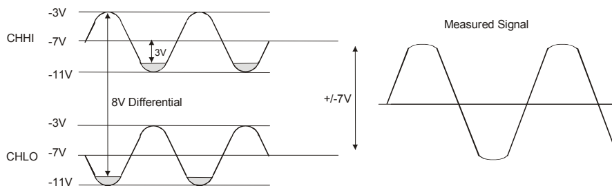
Figure 9. Differential voltage example: common mode voltage of -7\text{ V}
