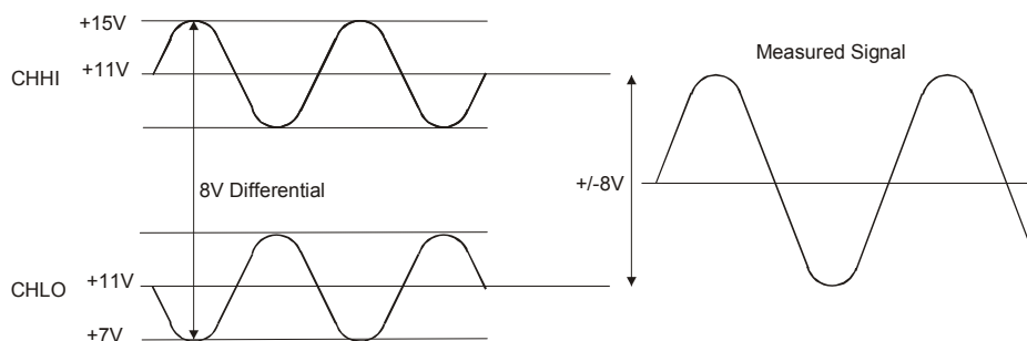
Figure 8. Differential voltage example: common mode voltage of 11\text{ V}
