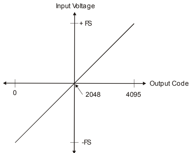
Figure 11. Ideal ADC transfer function
