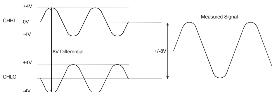
Figure 7. Differential voltage example: common mode voltage of 0\text{ V}
