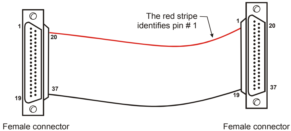
Figure 15. C37FF-x cable
