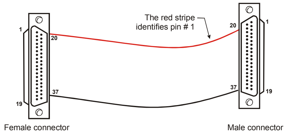
Figure 17. C37FM-x cable
