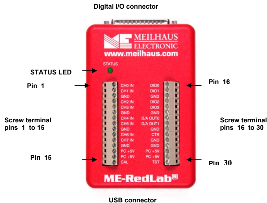
Figure 3. RedLab 1008 external components
