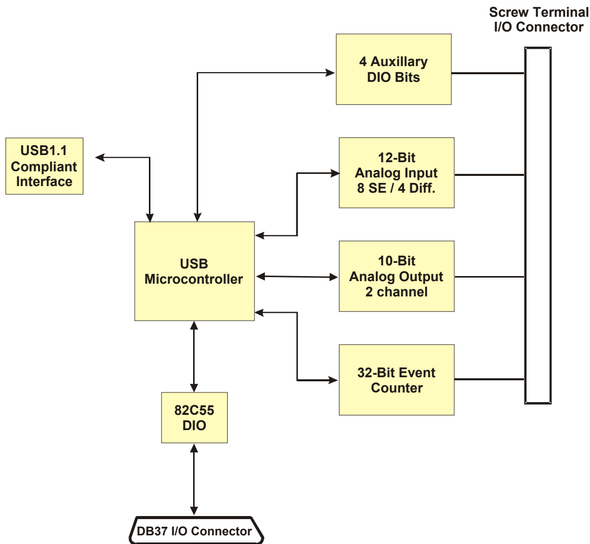
Figure 2. RedLab 1008 Functional Block Diagram
