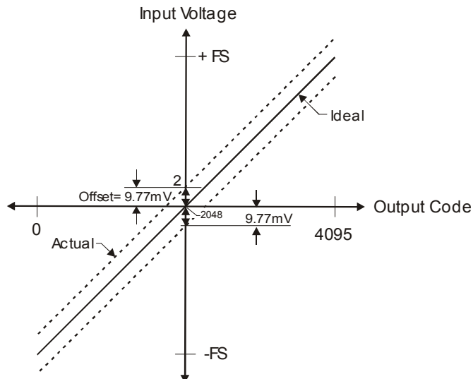
Figure 12. ADC transfer function with offset error
