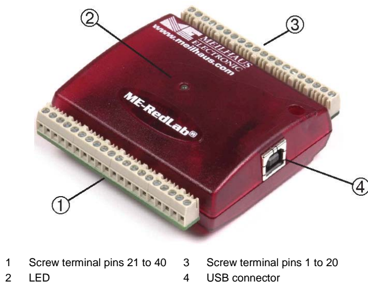
Figure 2. External components
