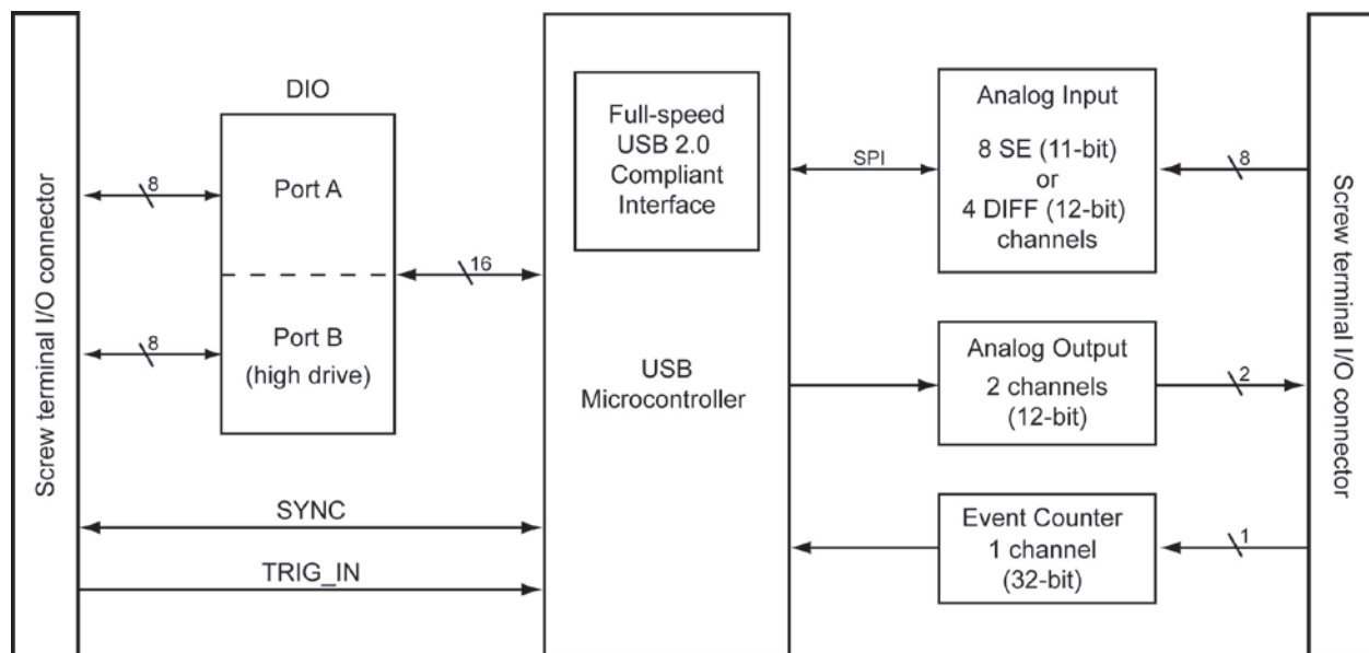
Figure 1. RedLab 1208FS-Plus functional block diagram
