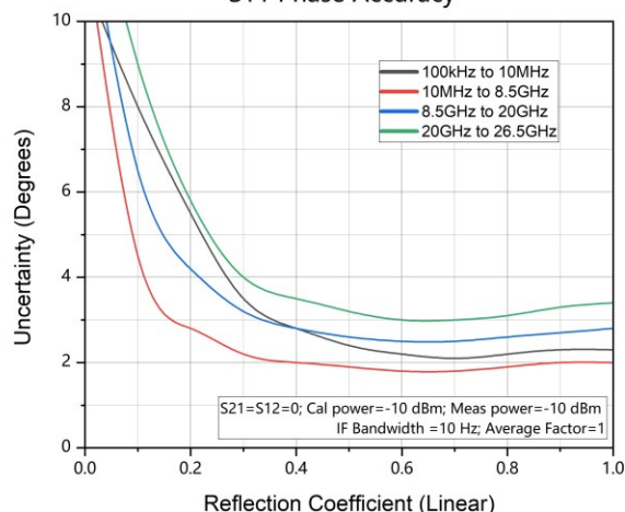
S11 Phase Accuracy
