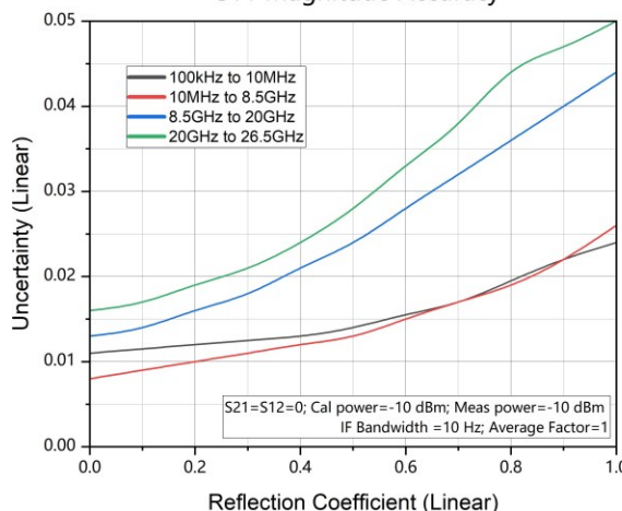
S11 Magnitude Accuracy
