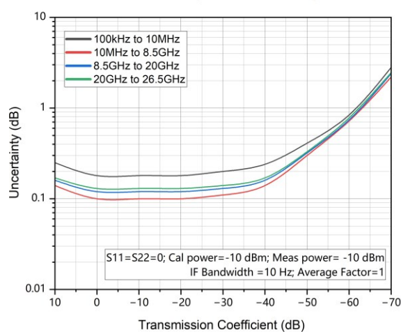
S21 Magnitude Accuracy
