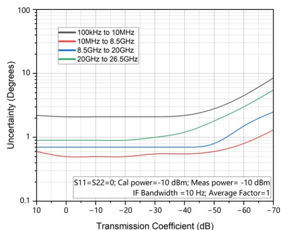
S21 Phase Accuracy
