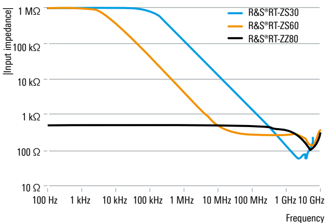
Input impedance versus frequency
