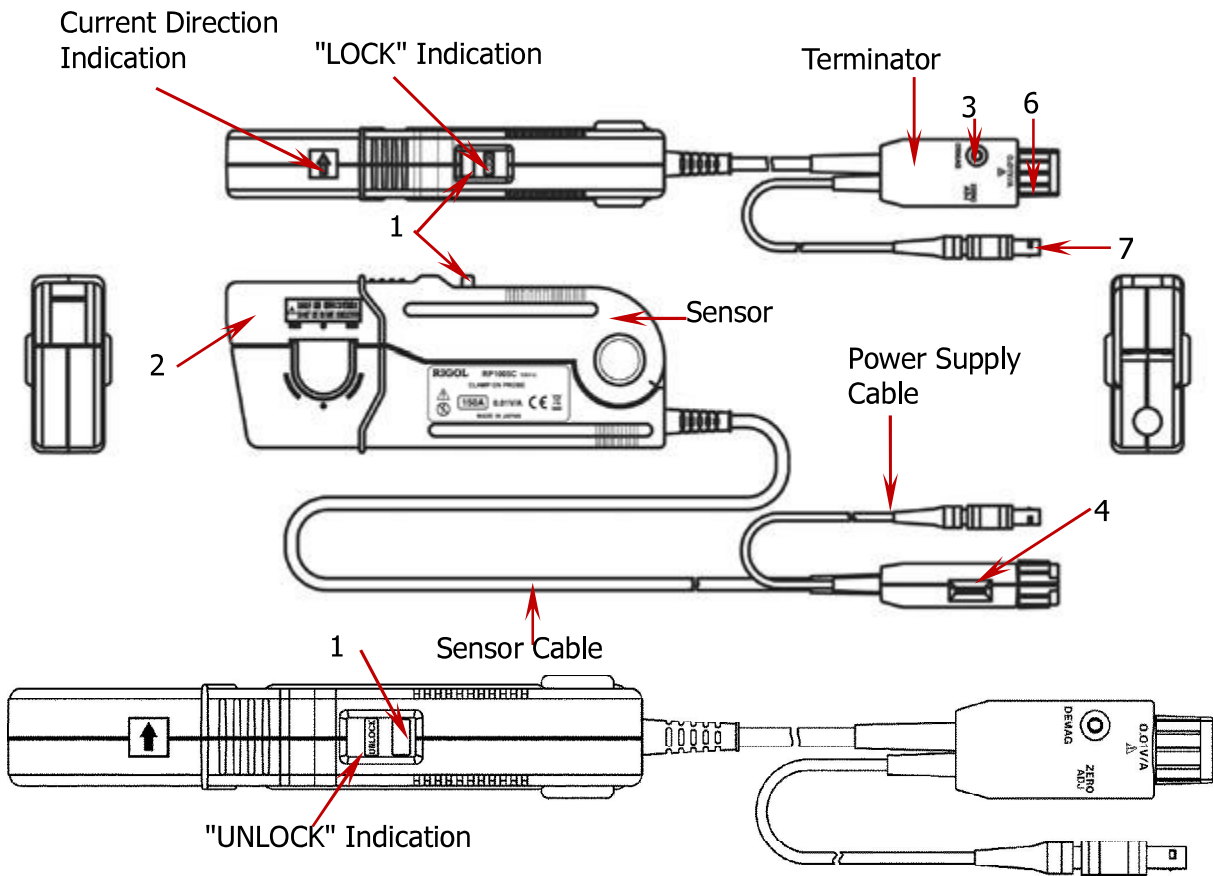
Figure 2 RP1005C/RP1006C Parts
