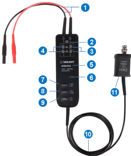
Figure 1 DPB6150A Probe View
