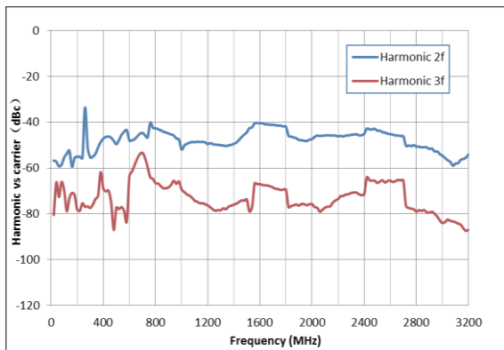
Measured harmonics versus carrier frequency at level \leq +13\text{ dBm}
