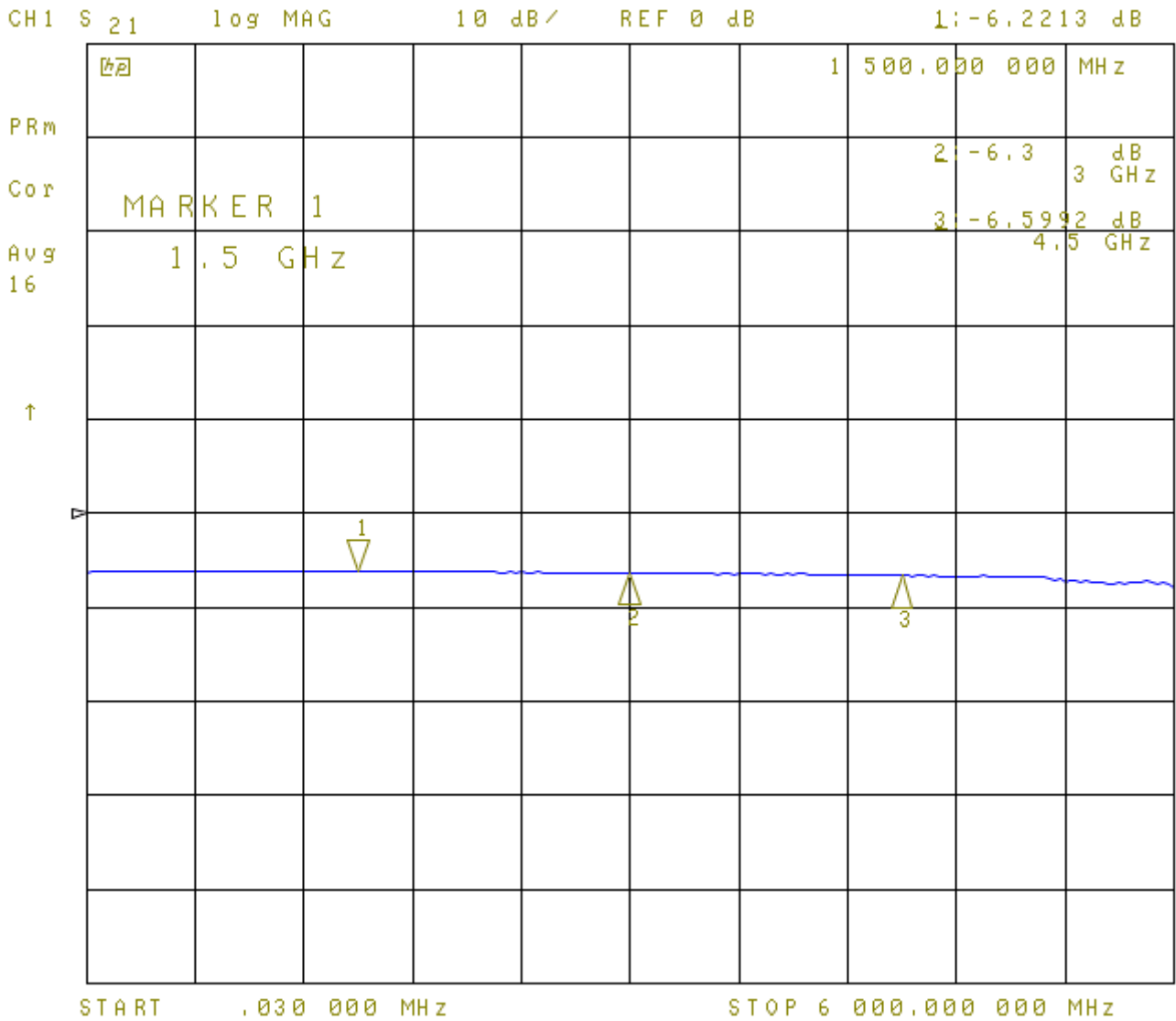
6dB Attenuator, S 21
