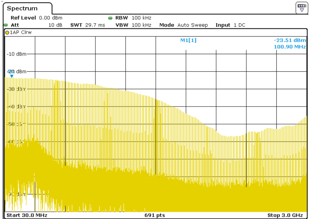
Figure 4 – 10 MHz comb frequency; amplifier on
