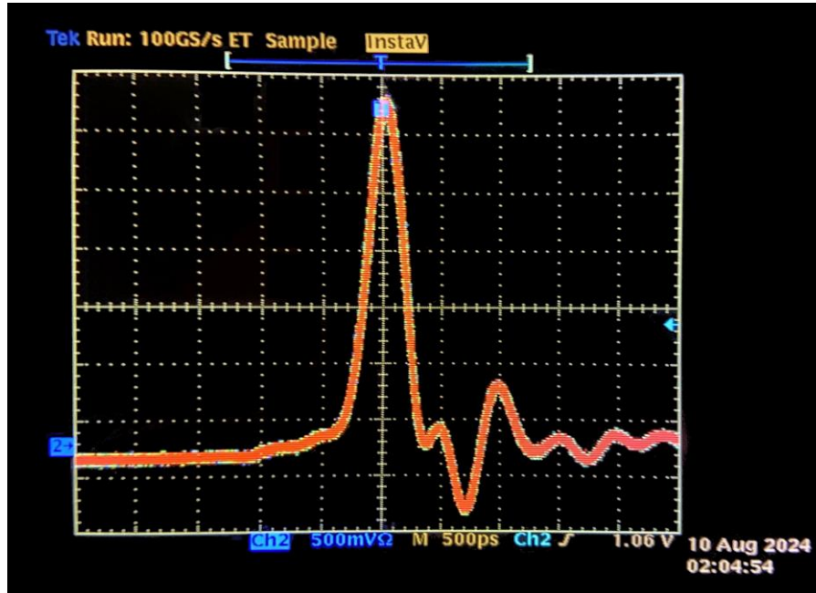
Picture 7: output pulse, 20 MHz base frequency, 50 \Omega termination
