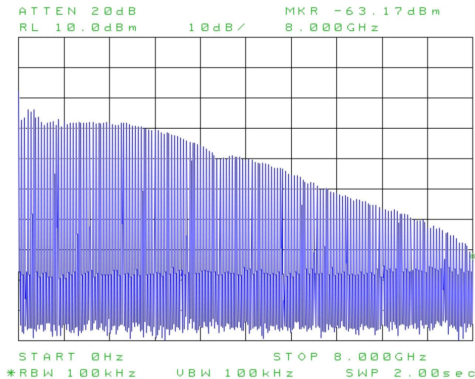
Picture 4: typ. comb spectrum, 0 – 8 GHz, 50 MHz base frequency
