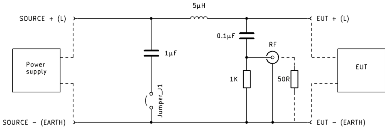
Figure 1: simplified schematic
