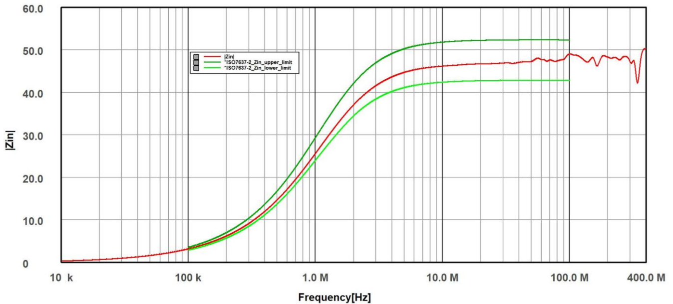
Figure 5: 100 kHz – 100 MHz, impedance of the TBL0510-1 5 \mu H LISN, ISO 7637-2 impedance*
