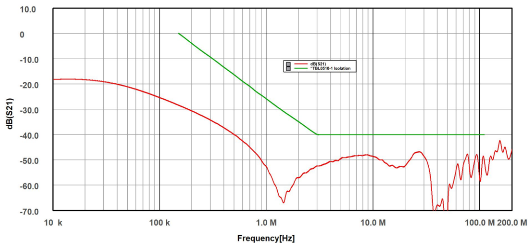
Figure 6: 150 kHz - 110MHz, isolation measured between DUT and source terminals; BNC connector terminated with 50 \Omega
