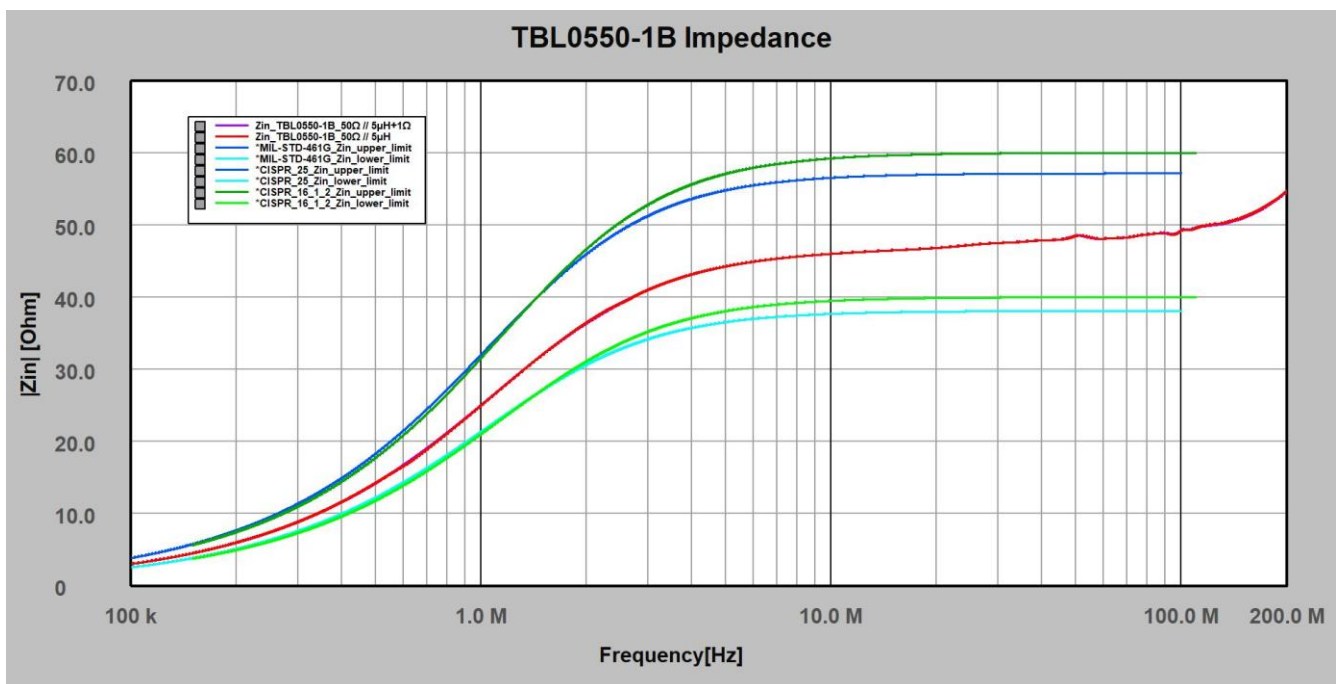
Figure 2: TBL0550-1B impedance , 100 kHz – 110 MHz, 50 \Omega // 5 \mu H+1 \Omega , 50 \Omega // 5 \mu H, source terminals shorted
