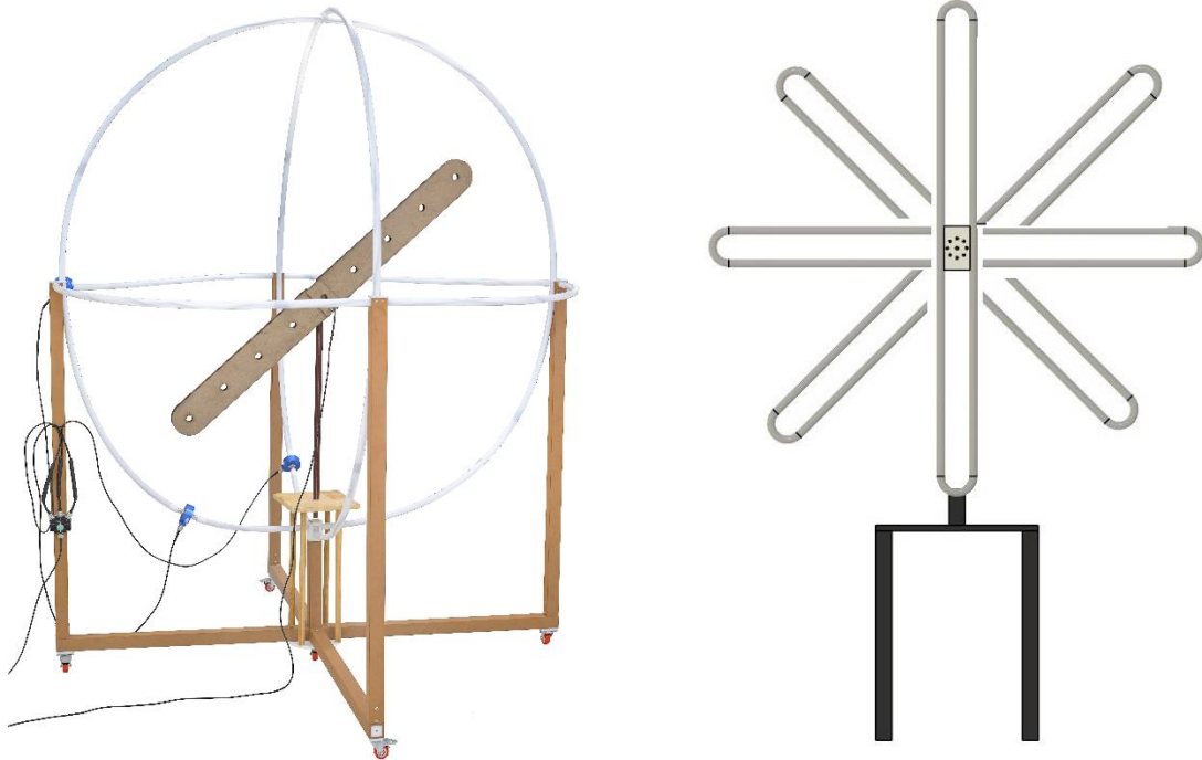
TBLLA-2M with calibration dipole TBLA-CDP
