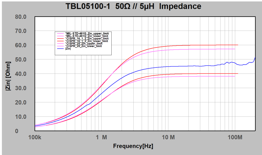
Picture 4: LISN impedance, 100 kHz – 110MHz; 50Ω // 5µH; Jumper J1 shorted, Jumper J2 open
