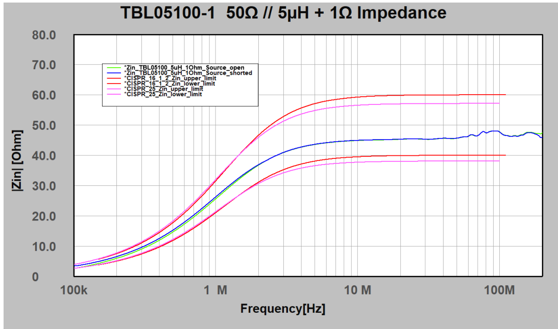
Picture 3: LISN impedance, 100 kHz – 110MHz; 50Ω // 5µH+1Ω; Jumper J1 open, Jumper J2 shorted
