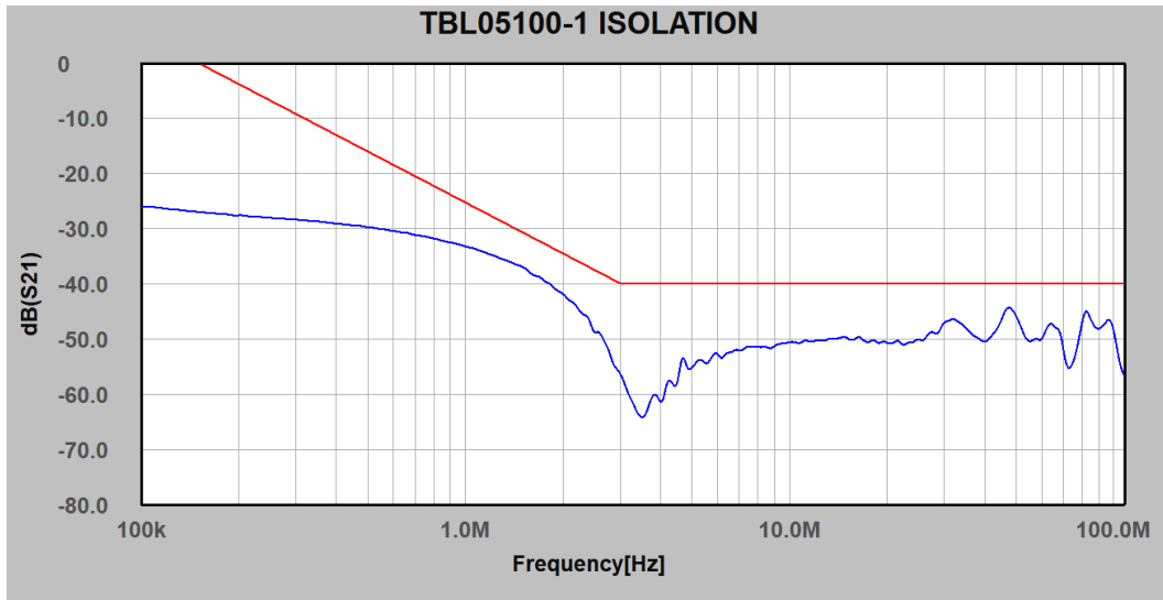
Picture 8: LISN Isolation, 100 kHz – 110MHz, 50Ω // 5µH+1Ω
