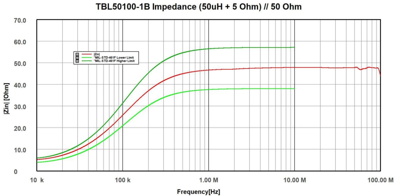
Picture 3: LISN impedance, (50 \mu H + 5 \Omega ) // 50 \Omega MIL-STD
